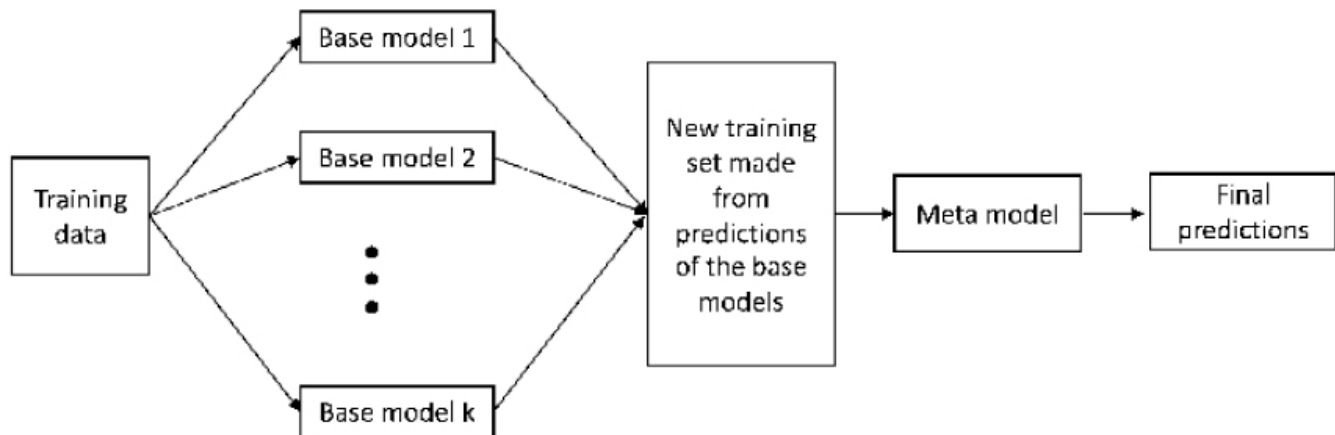
Figure 4. Stacking Algorithm
