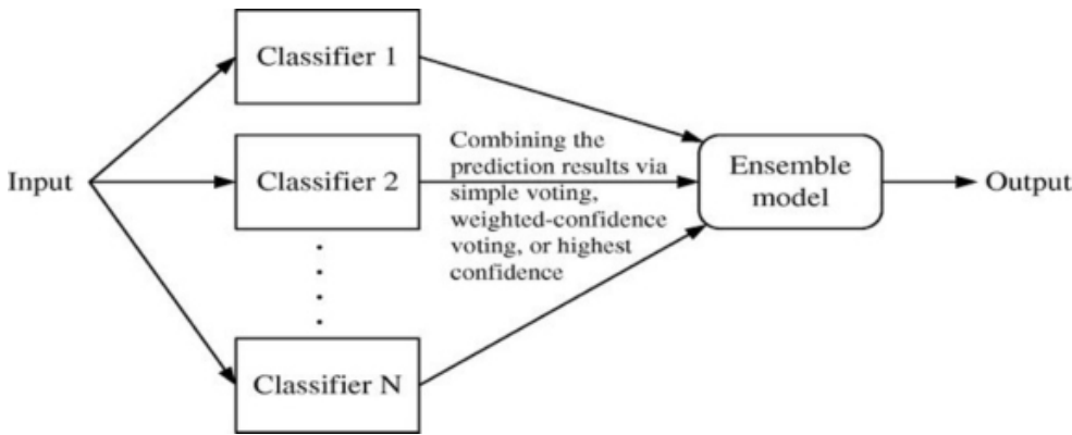
Figure 3. Voting Algorithm
